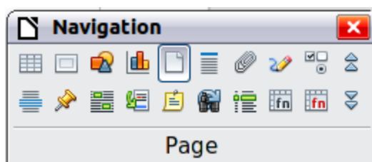
Figure 22: Navigation toolbar
