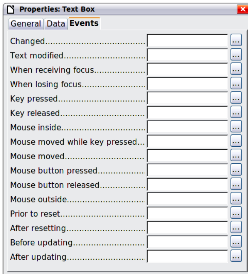
Figure 442: Control properties, Events tab
