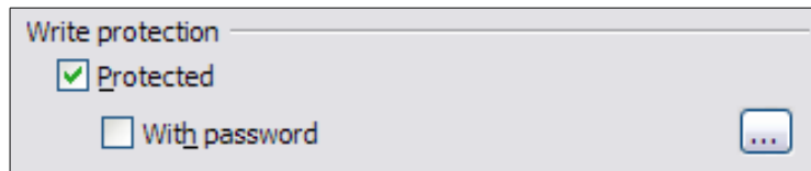
Figure 131: Write-protecting sections
