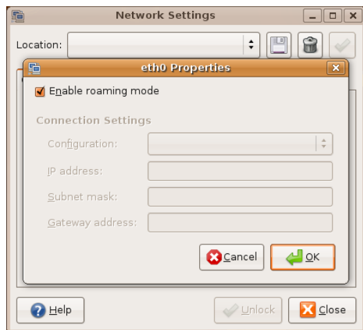
Figure 3.5. eth0 Properties
