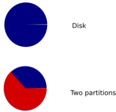
Figure 10.1. Partitioning
